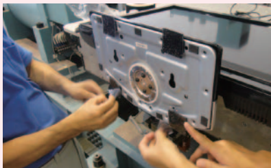
Install to stumble prevention sheet to 32-inch LCD TV.
