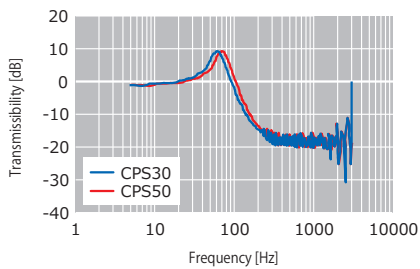
Test condition / Weight : 1.6kg Test pieces : Cushion pat S each hardness
