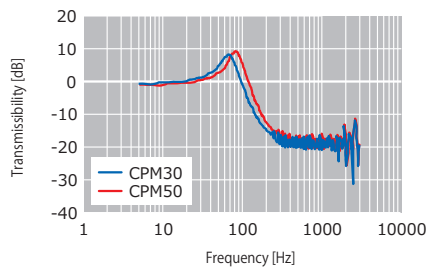
Test condition / Weight : 1.6kg Test pieces : Cushion pat M each hardness
